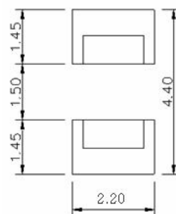
Recommended Solder Pattern
