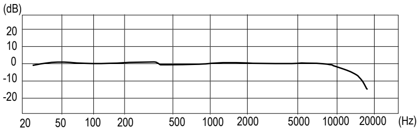
Typical free-field response 0° incidence
