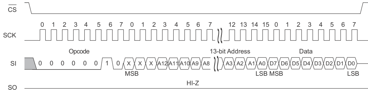
Figure 11. Memory Read
