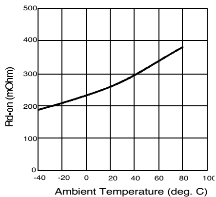
Figure 4. Typical On-Resistance
