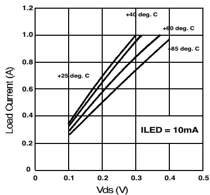
Figure 3. Typical On-Characteristics
