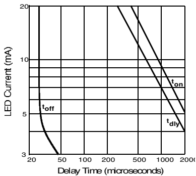
Figure 7. Typical Delay Times
