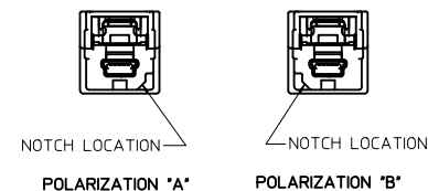
MINI-B PLUG POLARIZATION OPTIONS
