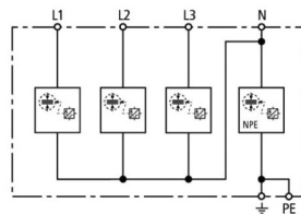
Basic circuit diagram I
