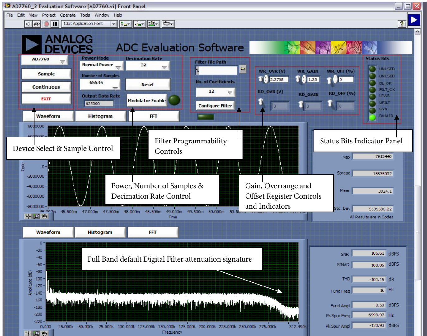
Figure 10. Front Panel GUI showing control and indicator information and the performance with a -0.5\text{ dB} 1\text{ kHz} input tone in decimate by 32 mode when running with the default 40\text{ MHz} MCLK.
