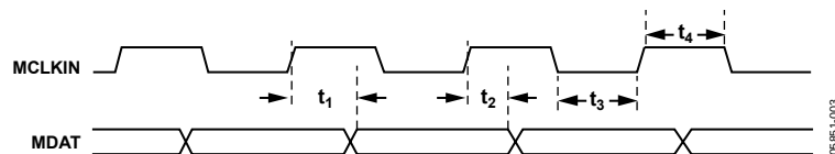
Figure 3. Data Timing
