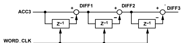
Figure 27. Differentiator
