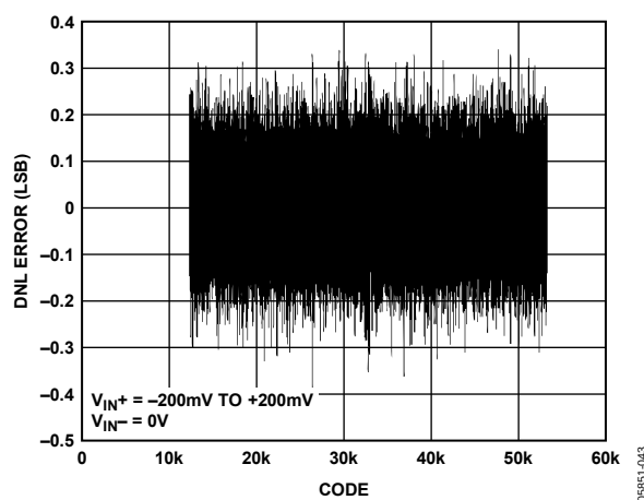
Figure 10. Typical DNL ( \pm 200\text{ mV} Range)
