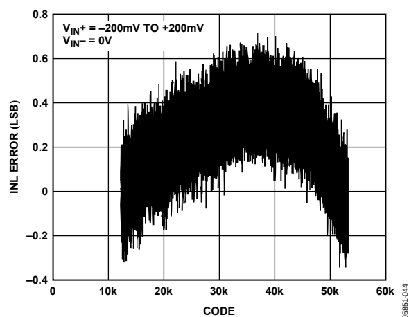
Figure 11. Typical INL ( \pm 200\text{ mV} Range)
