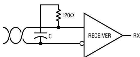
Figure 10. AC Coupled Termination
