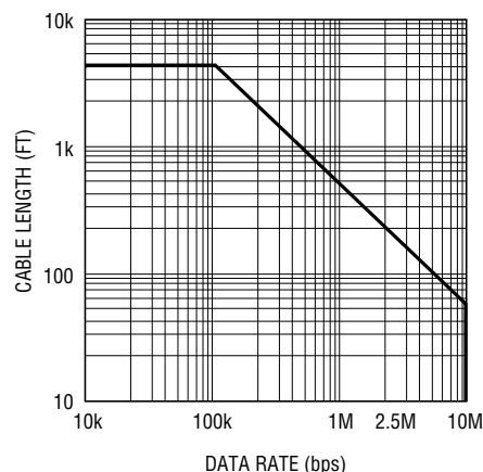
RS485 Cable Length Specification*
