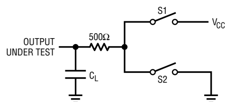
Figure 5. Driver Timing Test Load #2
