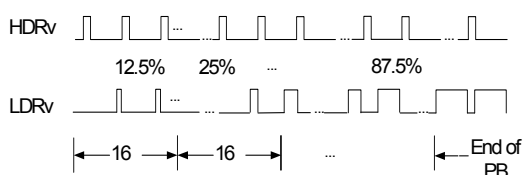
Figure 6b: Pre-Bias startup pulses
