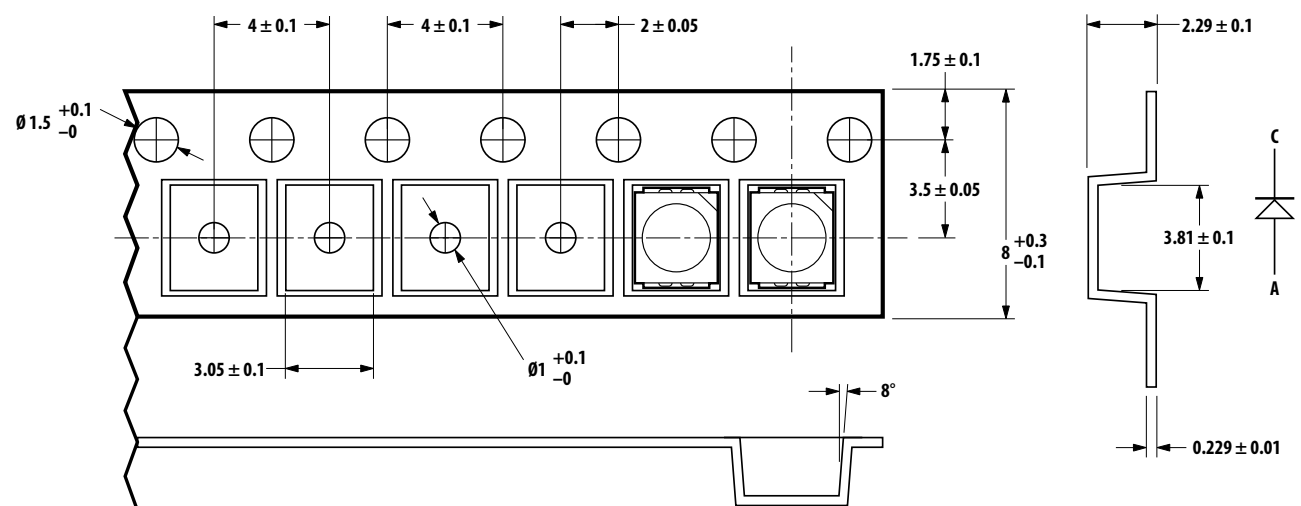
Figure 12. Tape dimensions
