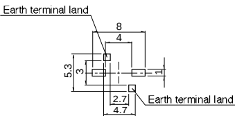
Printed circuit board land dimensions (When viewed from the switch mounting face)
