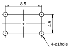
Printed circuit board mounting hole dimensions (When viewed from the switch mounting face)
