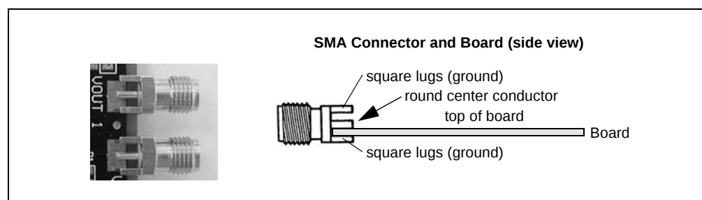
FIGURE 2-2: SMA Connectors.
