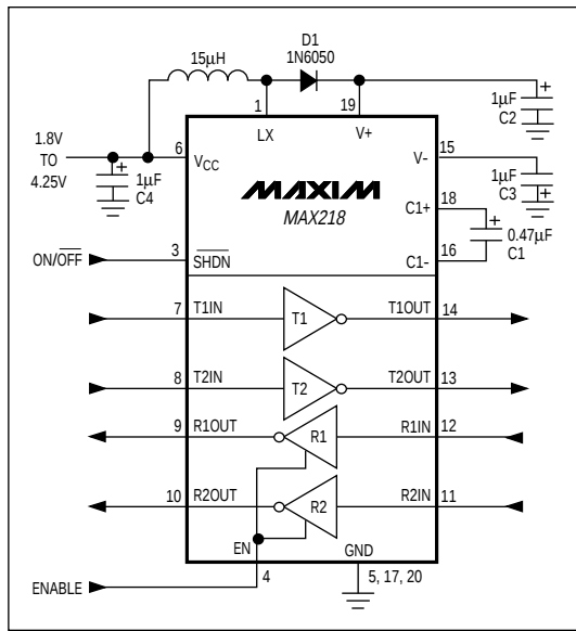
Figure 1. Single-Supply Operation
