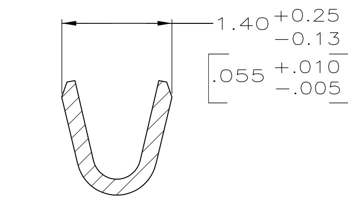
SECTION Y—Y WIRE BARREL SCALE 20:1
