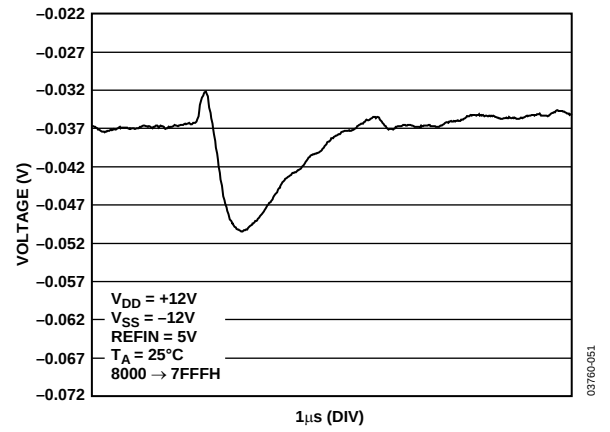
Figure 33. Major Code Transition Glitch Energy, \pm 12 V Supplies
