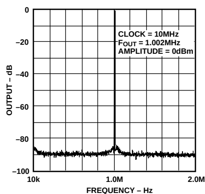
Figure 17. Typical SFDR (With a Window)
