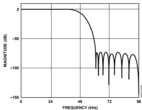
Figure 8. DAC Stop-Band Filter Response, 96 kHz
