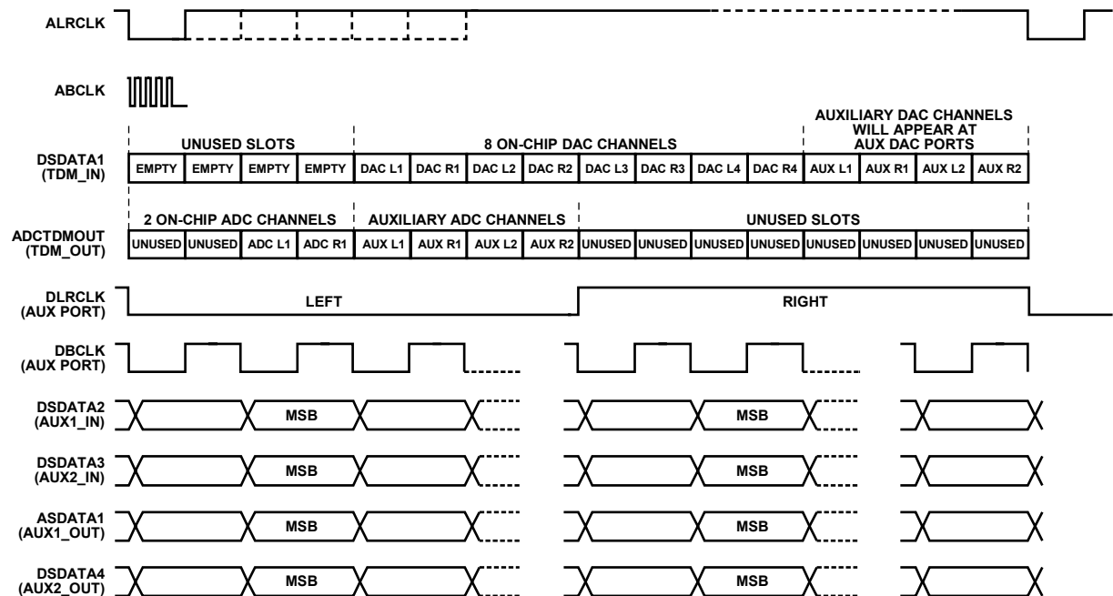
Figure 17. Combined AUX DAC and ADC Mode
