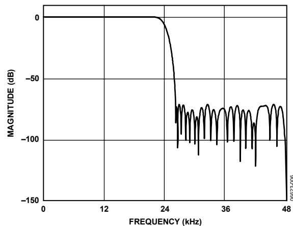
Figure 6. DAC Stop-Band Filter Response, 48 kHz
