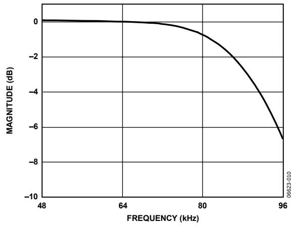
Figure 10. DAC Stop-Band Filter Response, 192 kHz
