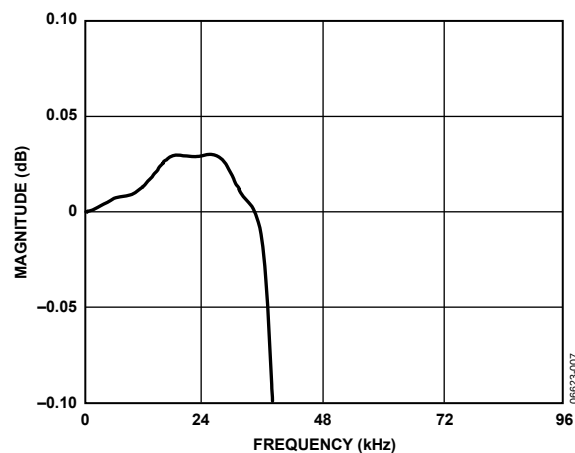
Figure 7. DAC Pass-Band Filter Response, 96 kHz
