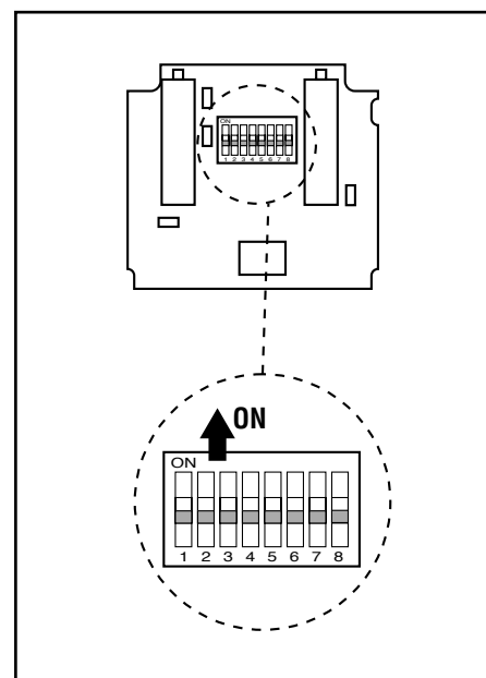
Figure 2. 45LM58 selection switch detail
