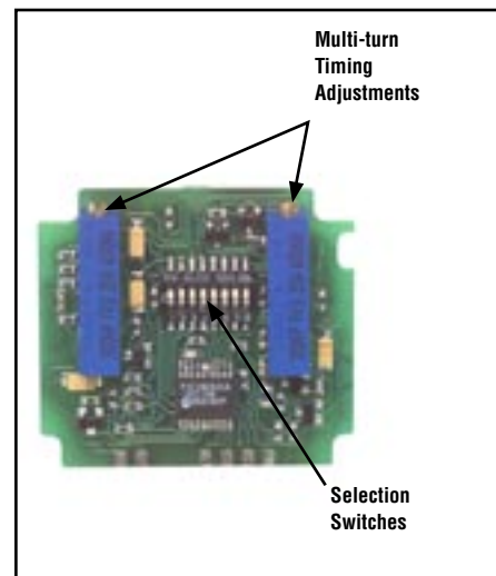
Figure 1. 45LM58 features
