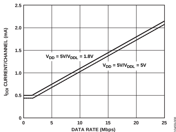
Figure 8. Typical V_{DDI} = 5 V Supply Current per Input Channel vs. Data Rate for 5 V and 1.8 V I/O Operation
