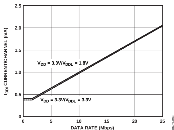
Figure 9. Typical V_{DDI} = 3.3 V Supply Current per Input Channel vs. Data Rate for 3.3 V, and 1.8 V I/O Operation
