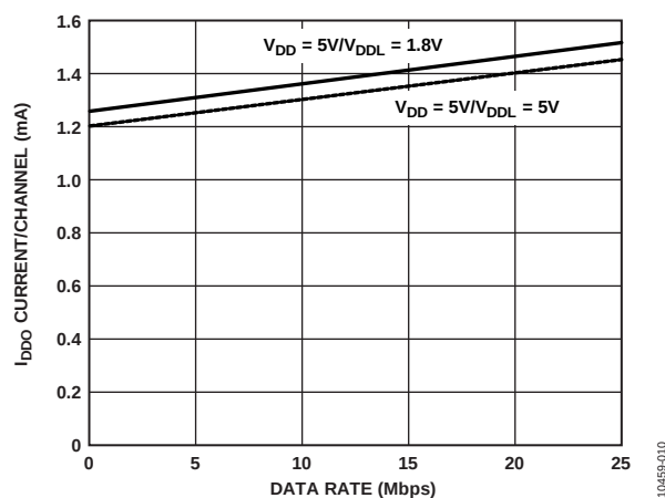
Figure 10. Typical V_{DDO} = 5 V Supply Current per Output Channel vs. Data Rate for 5 V and 1.8 V I/O Operation
