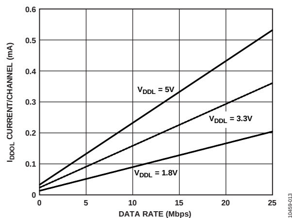
Figure 13. Typical V_{DDOL} Output Supply Current vs. Data Rate for 5 V, 3.3 V, and 1.8 V, C_L = 0 pF Operation
