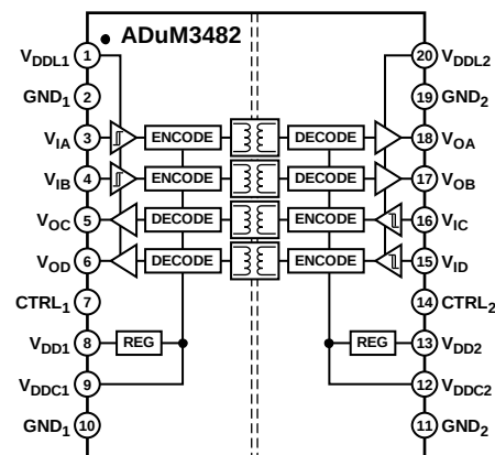
Figure 3. ADuM3482
