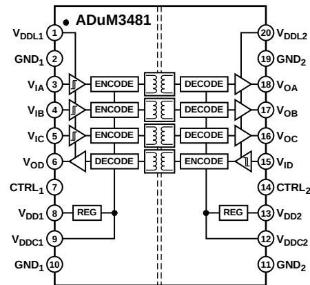
Figure 2. ADuM3481
