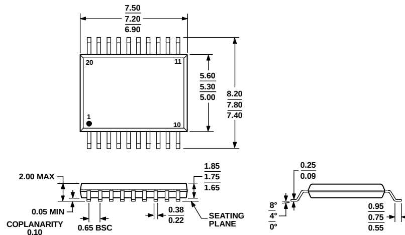
Figure 22. 20-Lead Standard Small Outline Package [SSOP] (RS-20)
