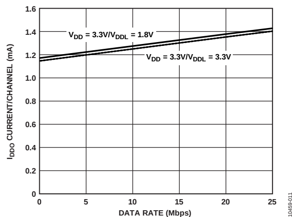
Figure 11. Typical V_{DDO} = 3.3 V Supply Current per Output Channel vs. Data Rate for 3.3 V and 1.8 V I/O Operation
