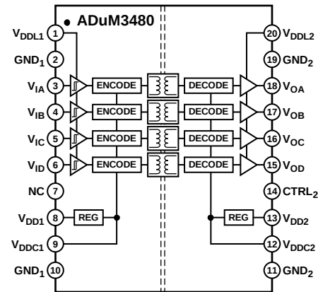
Figure 1. ADuM3480
