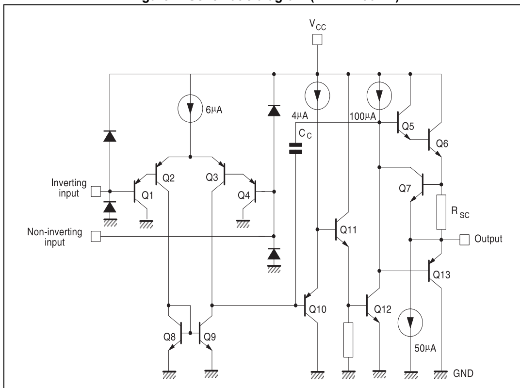
Figure 1. Schematic diagram (1/4 LM2902W)
