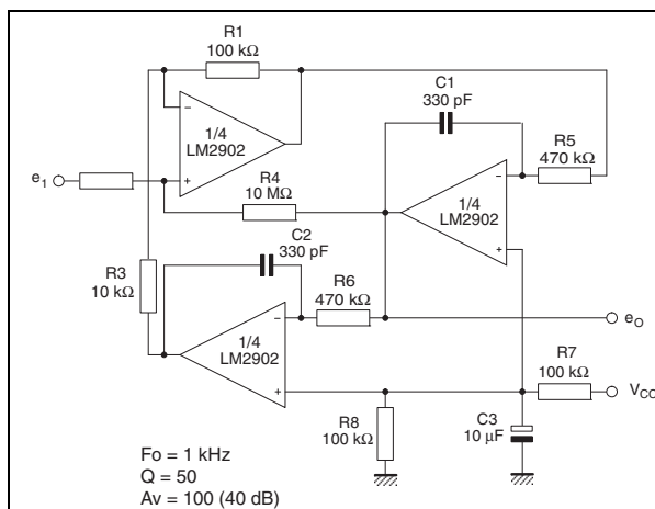
Figure 22. Active bandpass filter
