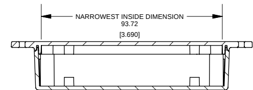
SECTION C-C
