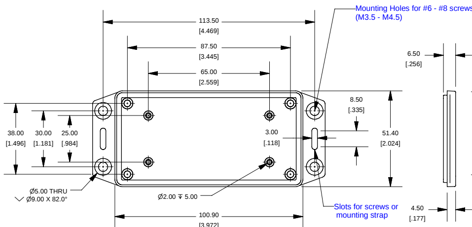
BOTTOM VIEW OF LID
