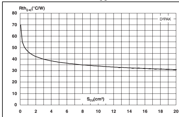
Figure 7. Thermal resistance junction to ambient versus copper surface under tab (Epoxy printed circuit board FR4, e_{CU} = 35 \mu m )
