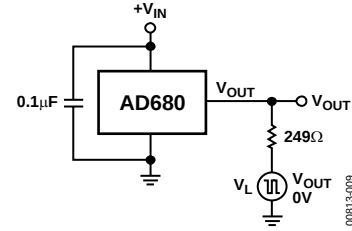
Figure 9. Transient Load Test Circuit
