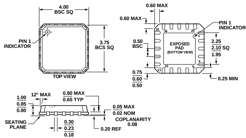
Figure 22. 20-Lead Lead Frame Chip Scale Package [LFCSP_VQ] 4 mm x 4 mm Body, Very Thin Quad (CP-20-1)
