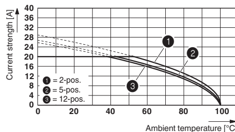
Derating curve for: PCC 4/...-ST-7,62 with PCVK 4-7,62
