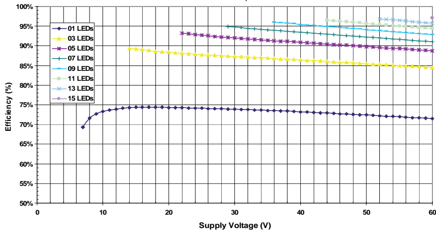
ZXLD1366 Efficiency L=220µH
