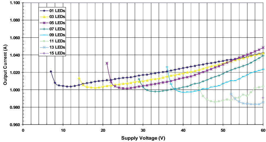
ZXLD1366 Output Current L=100μH
