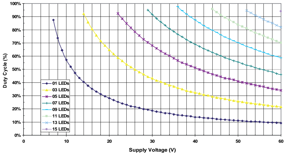
ZXLD1366 Duty Cycle L=220μH
