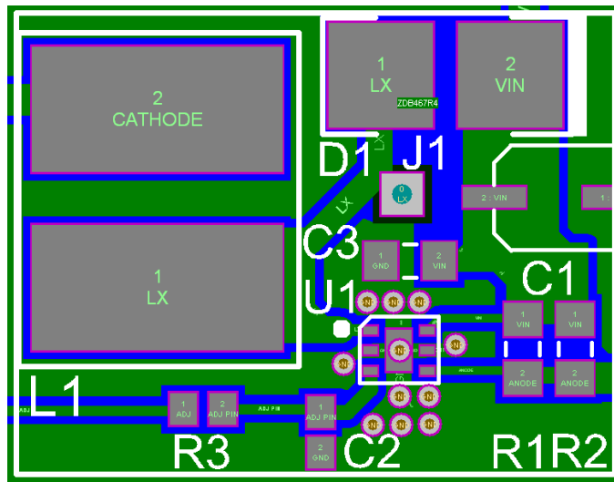
Figure 7. Suggested layout for DFN3030-6 package
