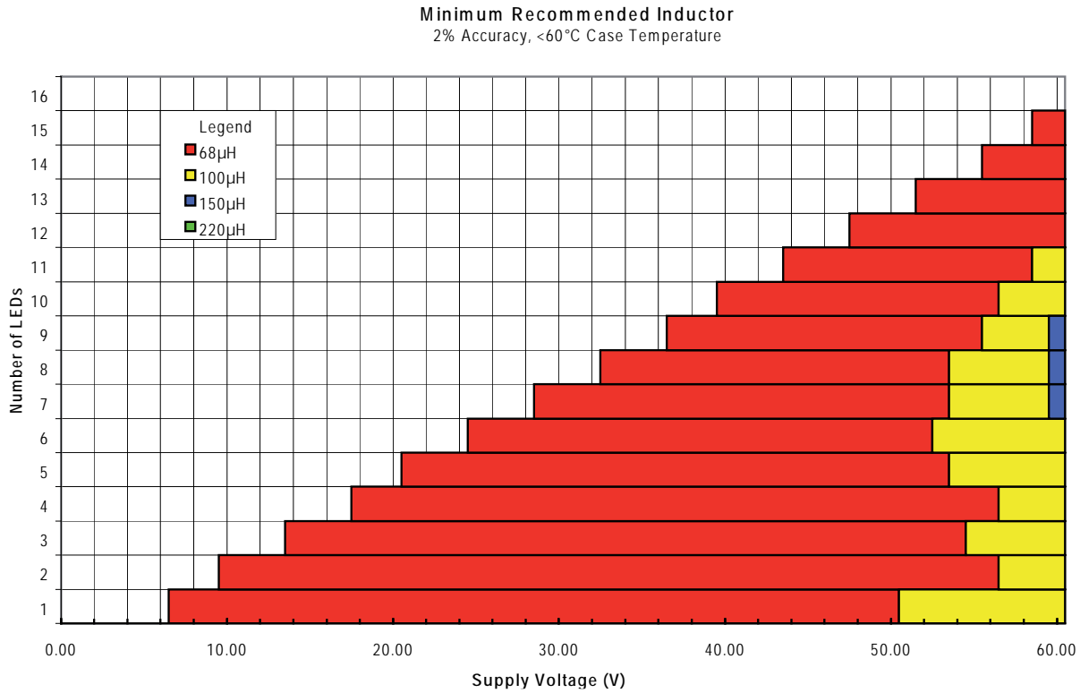
Figure 4. ZXLD1366 Minimum recommended inductor (DFN3030-6)
