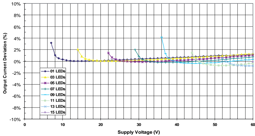
ZXLD1366 Output Current Deviation L=220µH
