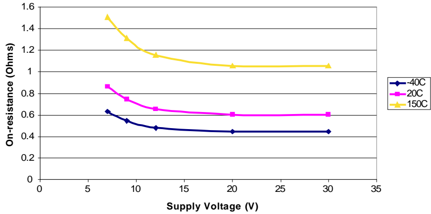
Lx on-resistance vs supply voltage
