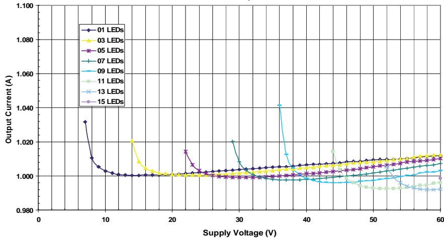
ZXLD1366 Output Current L=220µH
