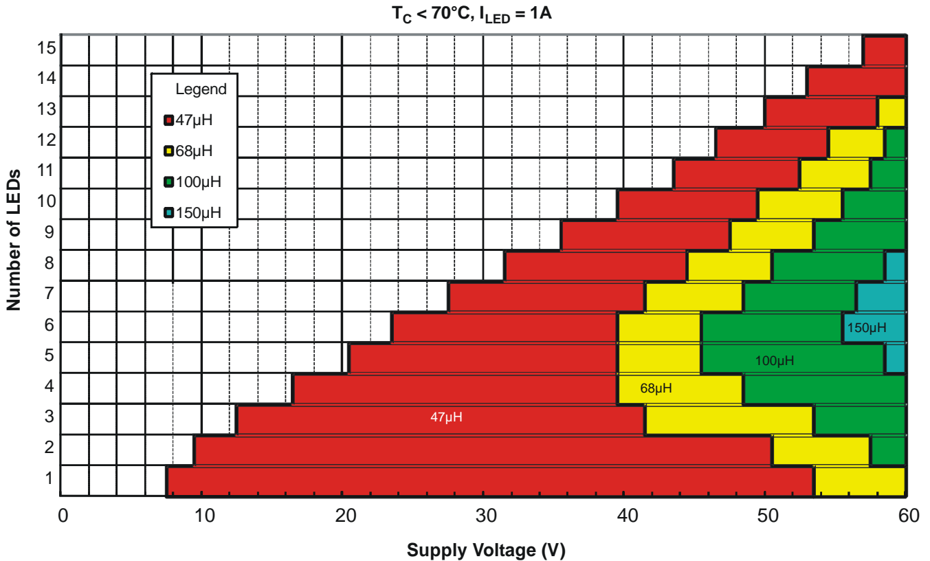
Figure 5. ZXLD1366 Minimum recommended inductor (SO-8EP)
