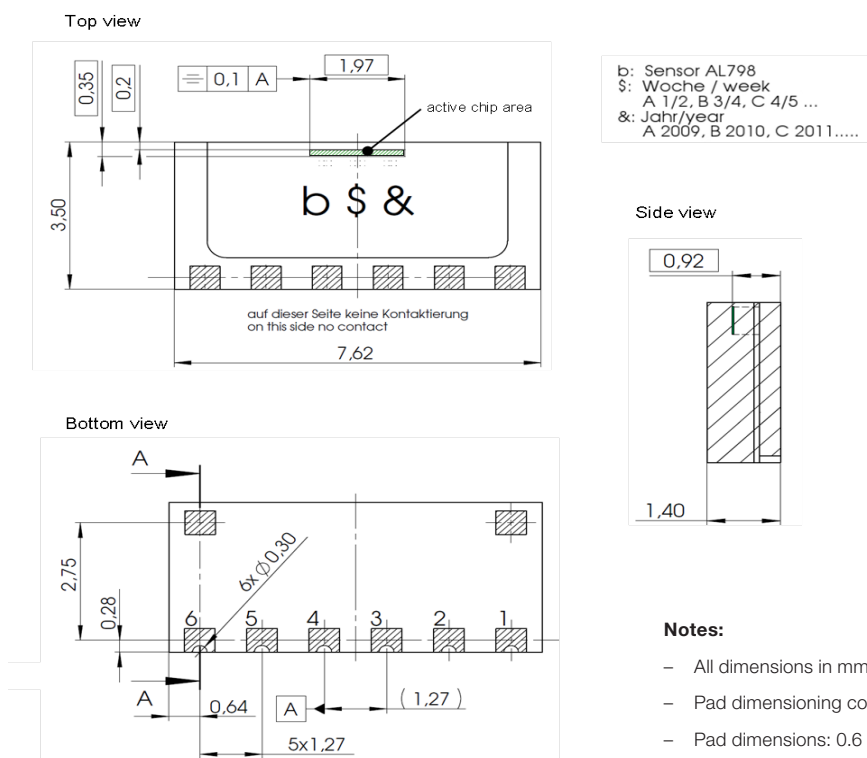
Fig. 7: SIL6 outline for AL798AKA.
