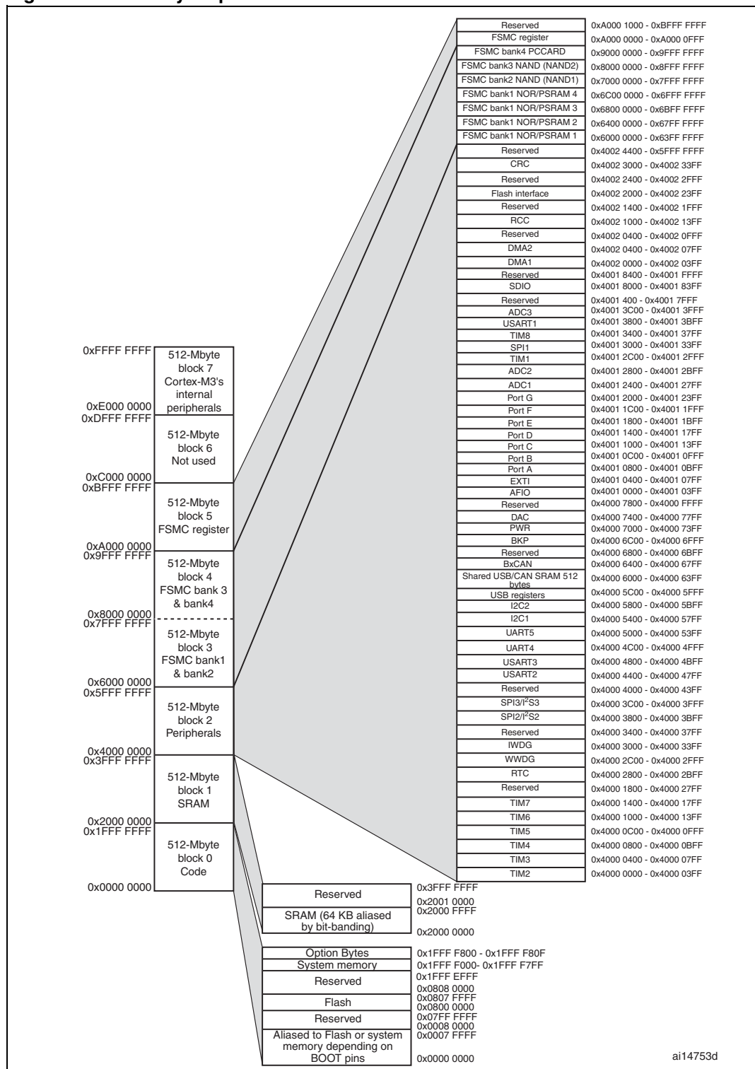
Figure 9. Memory map
