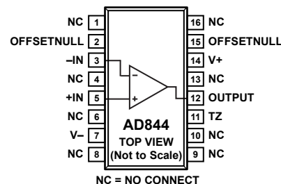
Figure 2. 16-Lead SOIC (R) Package
