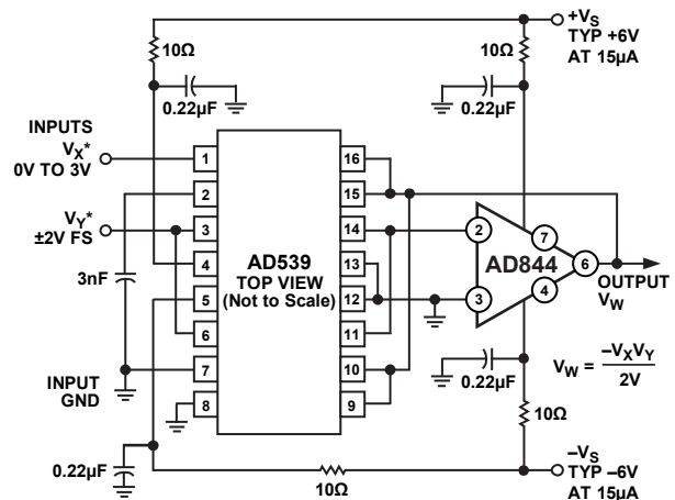
Figure 44. 20 MHz VGA Using the AD539
