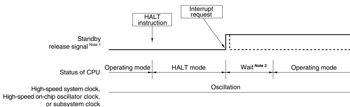
Figure 21-1. HALT Mode Release by Interrupt Request Generation
