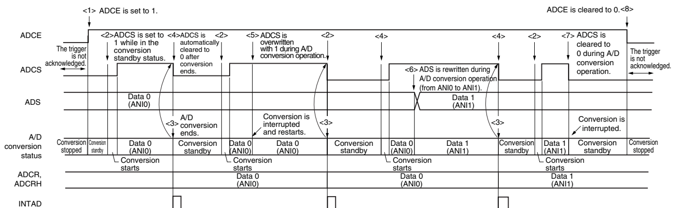
<R> Figure 12-18. Example of Software Trigger Mode (One-Shot Conversion Mode) Operation Timing
