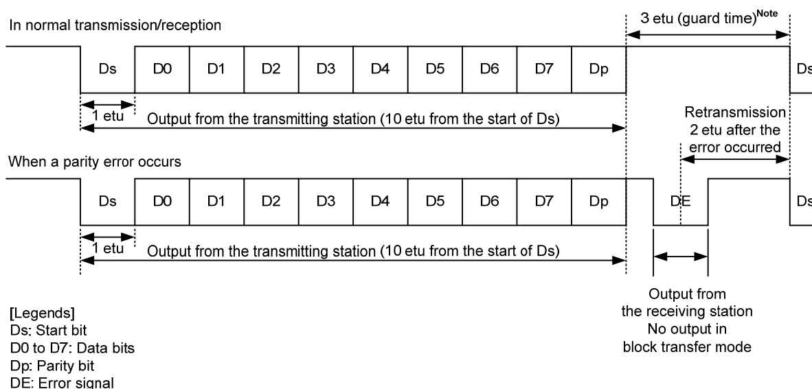
Figure 16-16. Data Format
