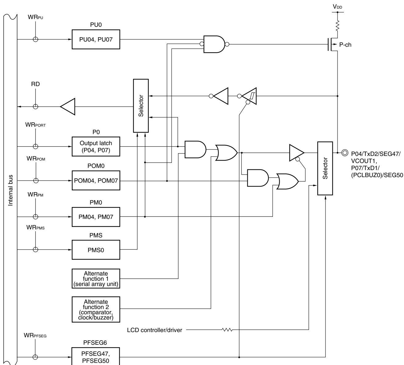
Figure 4-4. Block Diagrams of P04 and P07
