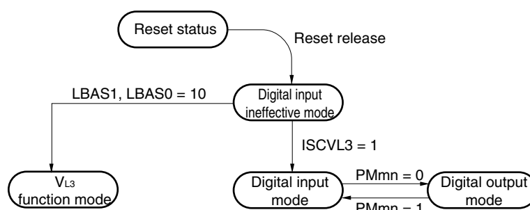
Figure 4-49. V L3 /P125 Pin Function Status Transition Diagram
