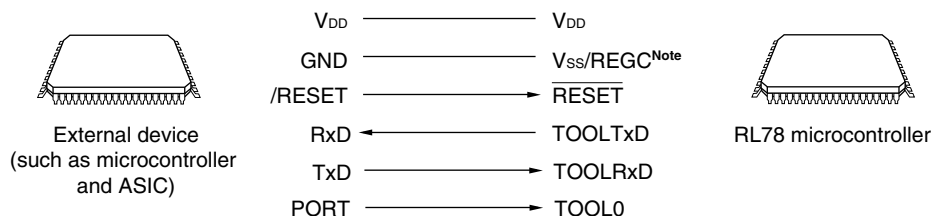
Figure 28-4. Communication with External Device
