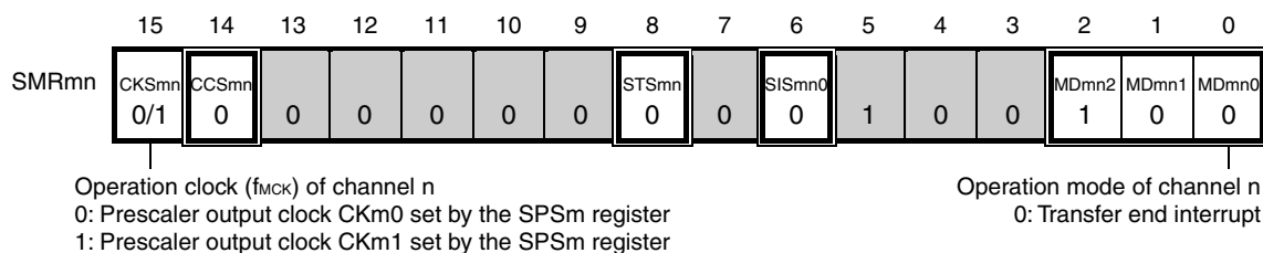
Figure 14-103. Example of Contents of Registers for Address Field Transmission of Simplified I 2 C (IIC00, IIC10) (1/2)
