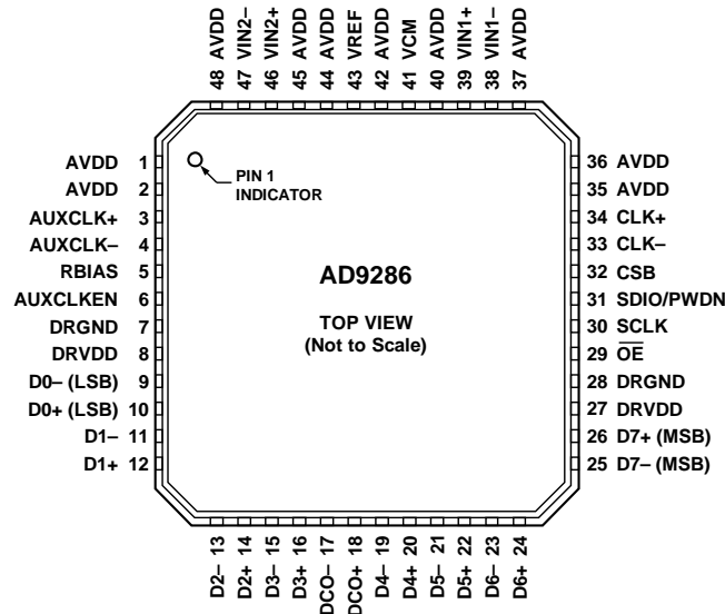
Figure 6. Pin Configuration
