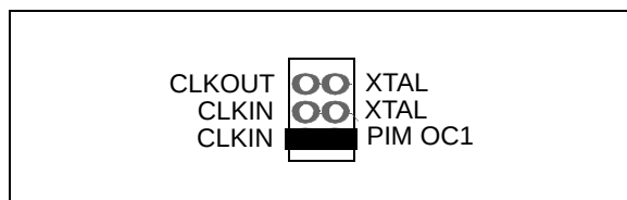
FIGURE 1-4: ADC Clock Selection Jumpers - Clock from MCU.
