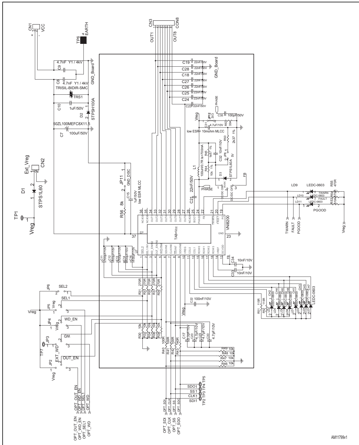
Figure 8. Typical circuit for switching regulation V_{DC-out} = 3.3 V
