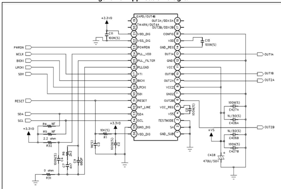
Figure 23. Application diagram
