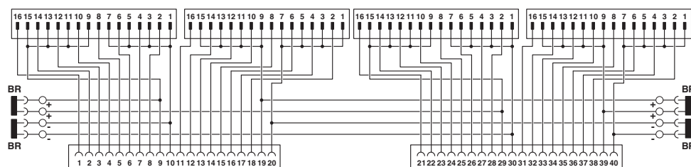
Circuit diagram
