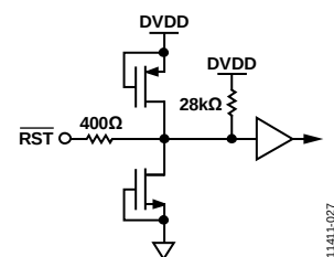
Figure 27. Equivalent \overline{RST} Input Circuit
