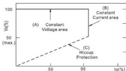
Typical LED power supply I-V curve
