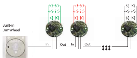
Example of a DimWheel wiring schematic
