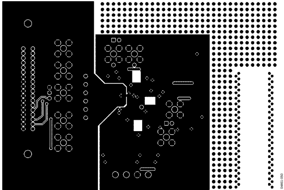
Figure 53. Solder-Side Artwork
