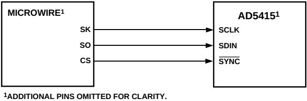
Figure 48. MICROWIRE-to-AD5415 Interface
