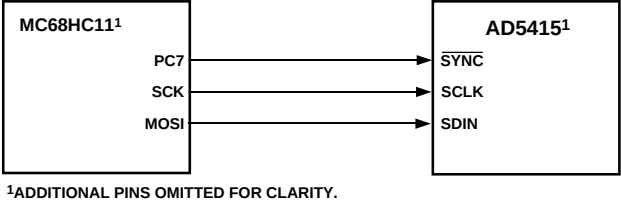
Figure 47. MC68HC11-to-AD5415 Interface
