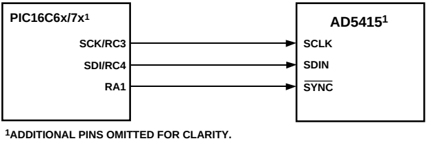
Figure 49. PIC16C6x/7x-to-AD5415 Interface
