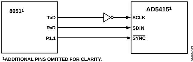
Figure 46. 80C51/80L51-to-AD5415 Interface
