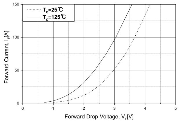
Fig.10 Forward Characteristics
