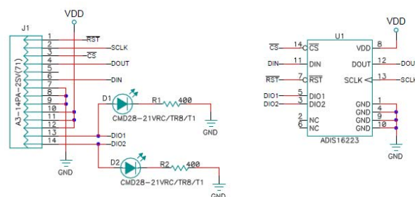
Figure 19. Electrical Schematic
