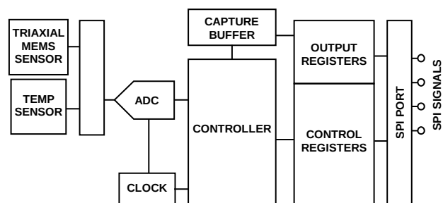
Figure 6. Simplified Sensor Signal Processing Diagram
