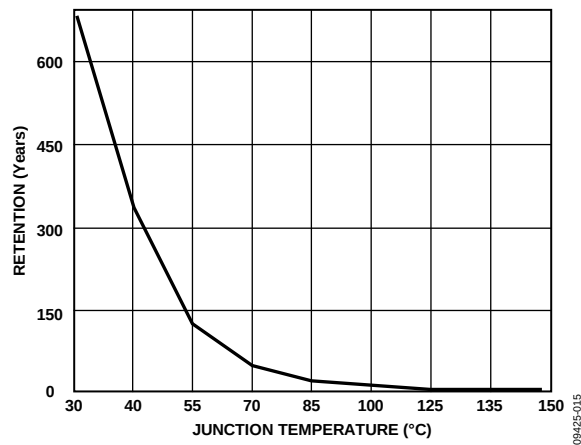
Figure 18. Flash/EE Memory Data Retention
