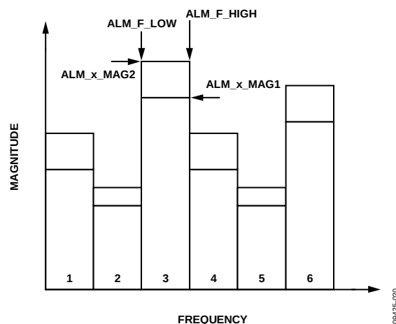
Figure 14. Spectral Band Alarm Setting Example, ALM_PNTR = 0x03
