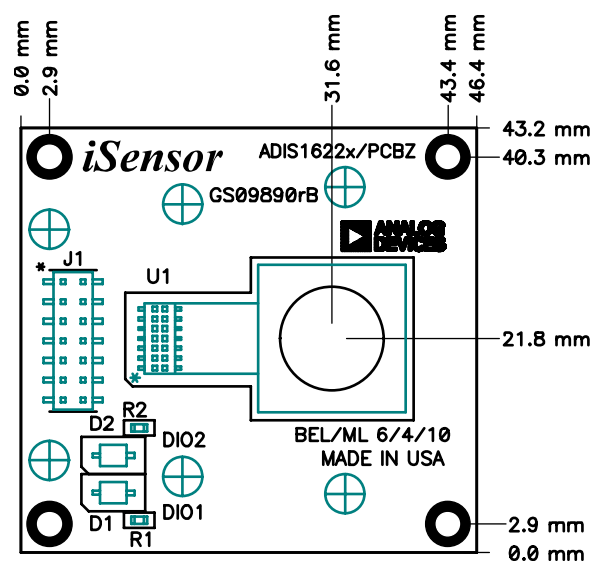
Figure 20. PCB Assembly View and Dimensions
