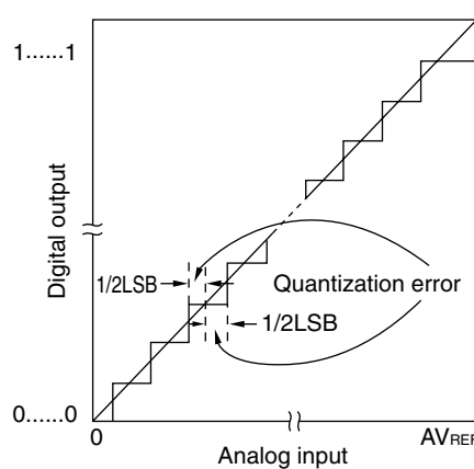
Figure 10-16. Quantization Error
