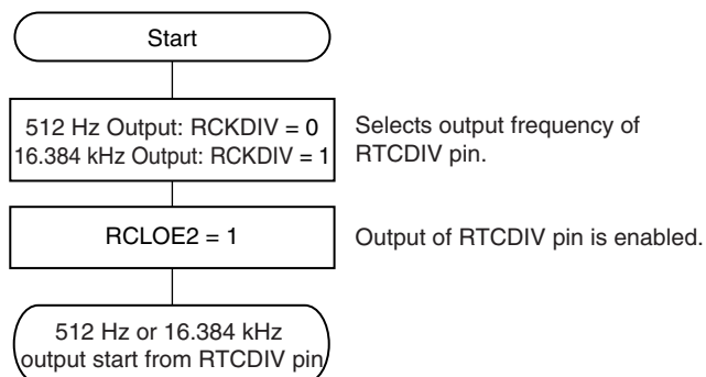
Figure 7-24. 512 Hz, 16.384 kHz output Setting Procedure
