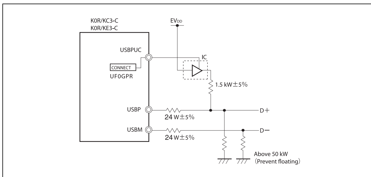
Figure 13-3. Example of USB Function Controller Connection
