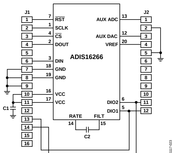
Figure 22. Electrical Schematic
