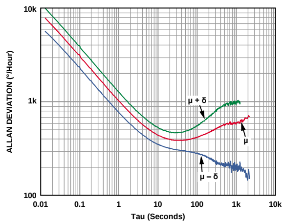
Figure 6. Allan Variance Plot
