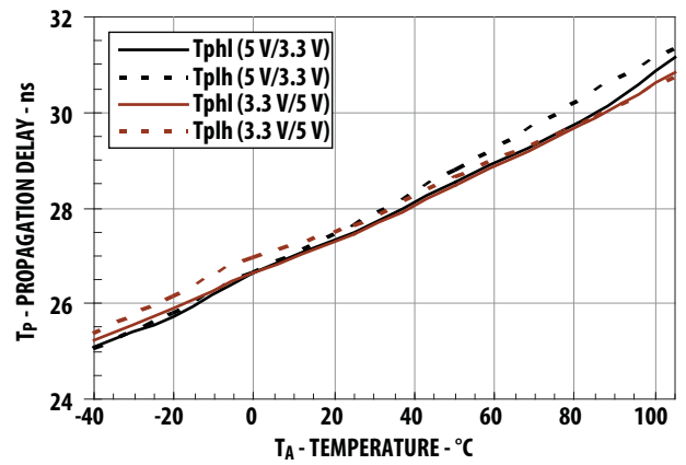
Figure 10. Typical Propagation Delay vs Temperature
