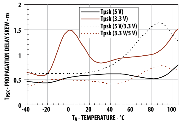
Figure 12. Typical Channel-Channel Delay Skew vs Temperature
