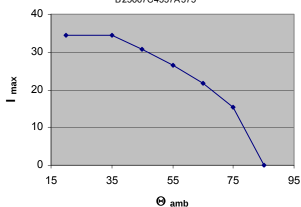
Max. allowable current (rms) at specific ambient Temp. B25667C4337A375
