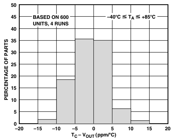
TPC 4. T_C - V_{OUT} Distribution
