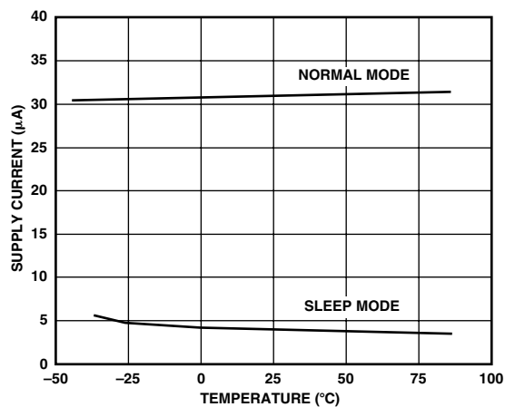
TPC 5. Quiescent Current vs. Temperature
