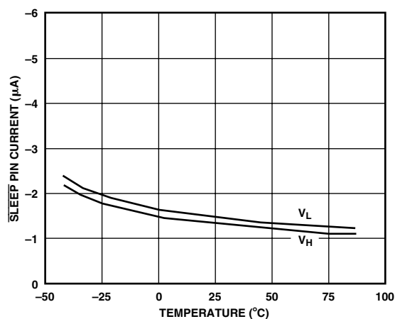
TPC 6. \overline{SLEEP} Pin Current vs. Temperature
