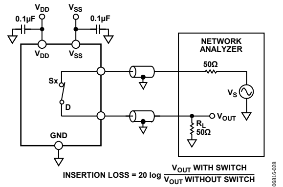
Figure 26. Bandwidth
