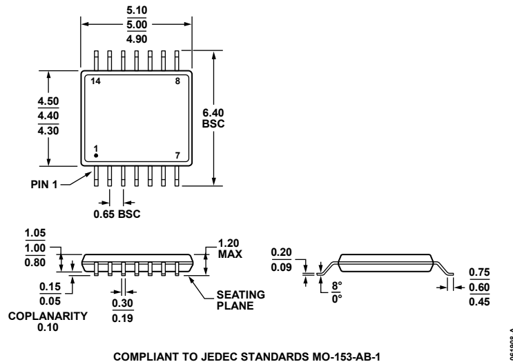
Figure 33. 14-Lead Thin Shrink Small Outline Package [TSSOP] (RU-14) Dimension shown in millimeters
