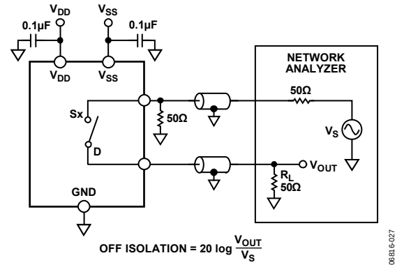
Figure 25. Off Isolation
