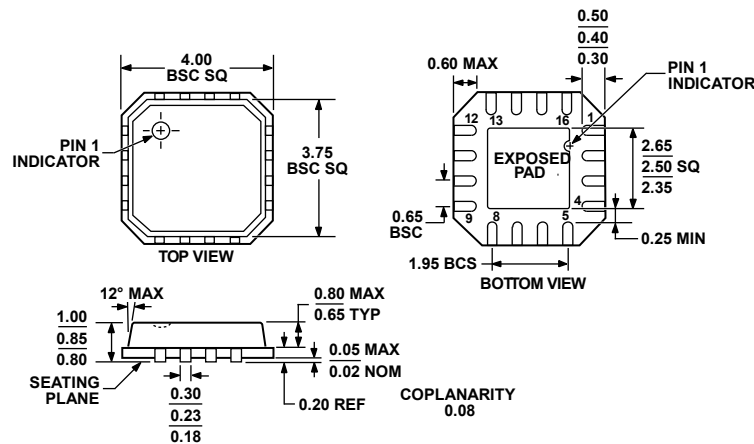
Figure 34. 16-Lead Lead Frame Chip Scale Package [LFCSP_VQ] 4 mm × 4 mm Body, Very Thin Quad (CP-16-13) Dimensions shown in millimeters
