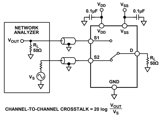
Figure 27. Channel-to-Channel Crosstalk
