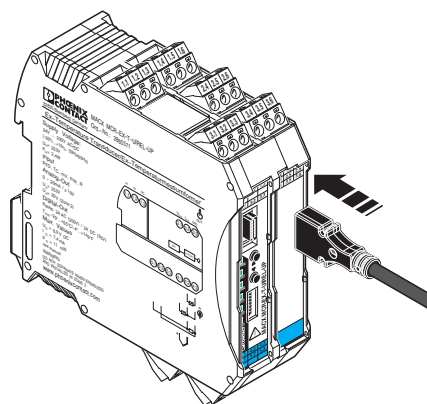
Figure 10 IFS-USB-PROG-ADAPTER
