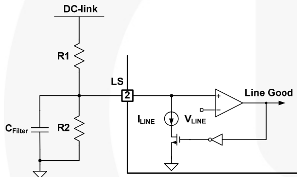
Figure 39. Line-UVLO
